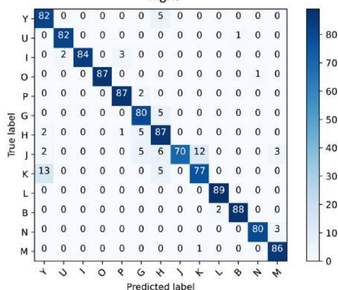
Extended Data Fig. 8 | Prediction of full keyboard. a , Each hand taking charge for the left half and right half of the keyboard. b , Confusion matrix of left side of keyboard. c , Confusion matrix of right part of keyboard. (Five-shot demonstrations for each key for transfer training dataset, accuracy left: 93.1%, right 93.1%).
